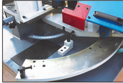
Swivel saw bow
