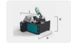
CUBO 350 NC BOX B 2000 mm L 2385 mm H 1610 mm h 880 mm Kg 950
